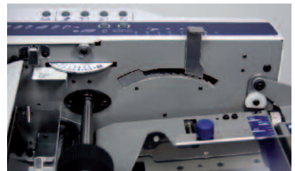
TF MEGA-A: Adjustment of the paper pressure and separation for different paper weights
